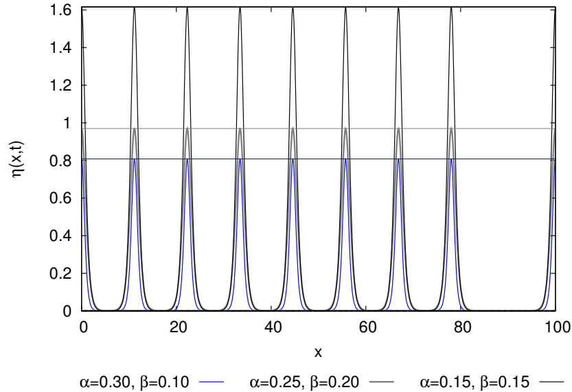
Fig. 10.13. Time evolution of the exact solitons \eta(x, t) = A \operatorname{Sech}^2(B(x - vt)) , according to the KdV2 equation (4.27) obtained in numerical simulations for three different sets of parameters \alpha and \beta . Reproduced with permission from [79]. Copyright (2014) by the American Physical Society
