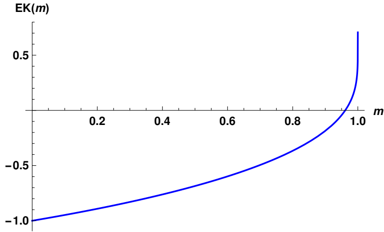
Fig. 5.1. Plot of the function EK(m) (5.14).
